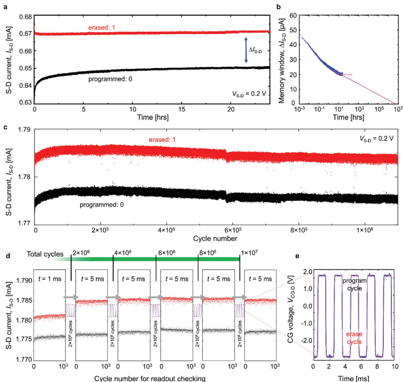
Figure 4. Retention and endurance characteristics. a) Retention data for a 20 μm gate-length cell. Program and erase cycles consisted of 10 ms duration pulses at +2.5 and −2.5 V, respectively. Readout is performed at an S-D bias of 0.2 V and in the absence of gate bias. b) S-D current difference ( \Delta I_{S-D} ) for the >24 h retention plotted on a log scale. The continuous magenta line indicates the most conservative interpretation of the decay data, whereas the dashed magenta line follows the stabilization of the memory window. c) Endurance data for continuous program-read-erase-read cycling (5 ms pulses) on a second 20 μm gate-length cell demonstrating a clear 0/1 contrast exceeding 10^6 cycles. d) Extended endurance to >10^7 cycles using continuous pulse trains of 2 \times 10^6 program-erase cycles repeated five times separated by 1000 program-read-erase-read cycles to confirm memory operation persists. The program and erase pulse duration, t , was 1 ms in the absence of read, and 5 ms with the read, except for the first set of 1000 program-read-erase-read cycles, where it was also 1 ms. The data are presented chronologically from left to right with the total cycles counted by the green bar. e) Oscilloscope trace showing the applied gate bias for a section of the pulse train during t = 1 ms program-erase endurance cycling.
